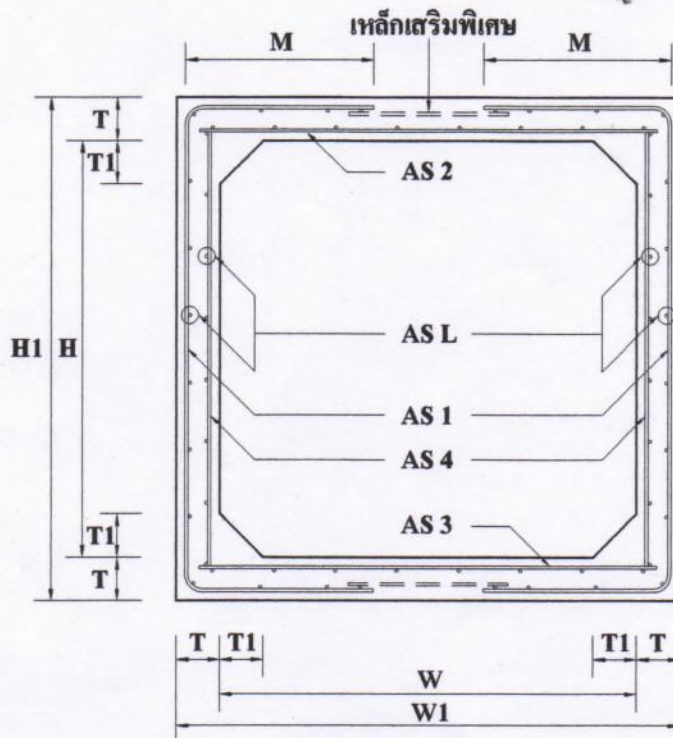
DETAIL FOR PRECAST BOX CULVERT
